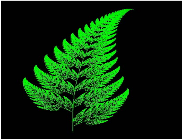
Iterated Function System (IFS) Fern
